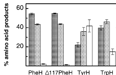
Figure 1. Product distribution with 4-CH 3 -phenylalanine as substrate for the aromatic amino acid hydroxylases: 4-HOCH 2 -phenylalanine (dark gray), 3-CH 3 -4-HO-phenylalanine (light gray), and 3-HO-4-CH 3 -phenylalanine (white). Reactions were carried out and the products analyzed by HPLC as described in ref 6. Conditions: 25 mM sodium phosphate buffer, pH 7.0, 30 \mu\text{M} ferrous ammonium sulfate, 1.2 mM 4-CH 3 -phenylalanine, 10 \mu\text{M} enzyme, and 150 \mu\text{M} 6-methyltetrahydropterin at 30 °C.
