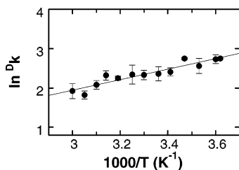
Figure 2. Deuterium kinetic isotope effects for benzylic hydroxylation as a function of temperature for \Delta 117\text{PheH} . Isotope effects were determined from the effects on product composition with 4\text{-C}^2\text{H}_3\text{-phenylalanine} . The line is from a fit to the Arrhenius equation.
